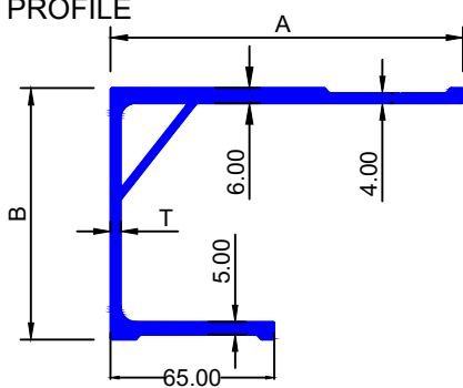
J-75 PROFILE
