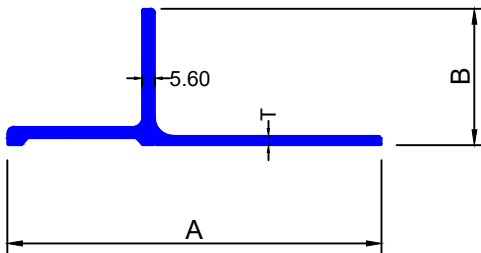
FLAT ANGLE -100
