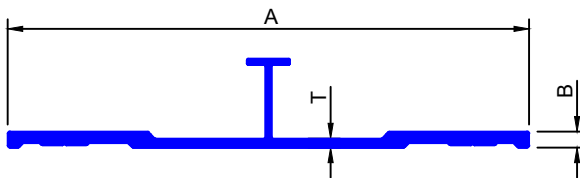
230T/BEAM BOTTOM 100
